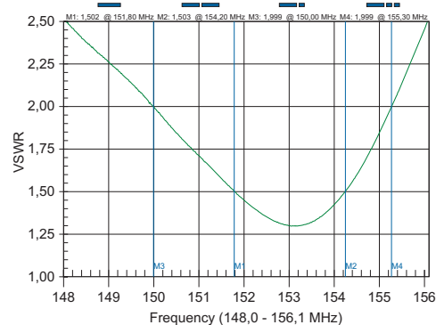
TYPICAL VSWR A-1000MV
